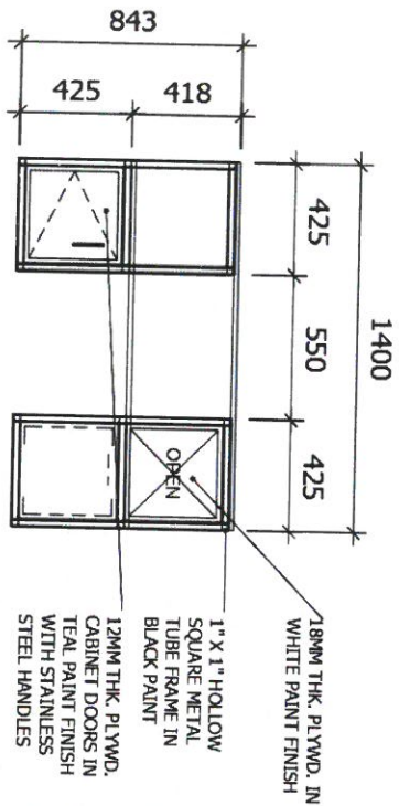
2 FRONT VIEW SCALE: 1:30M
