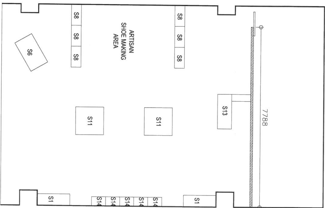
SCHEMATIC LAY-OUT (FELIZ MALL)
