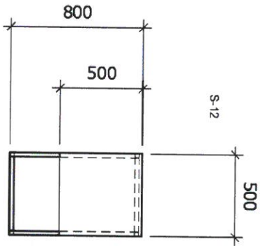
2 FRONT VIEW S-12 SCALE: 1:30M
