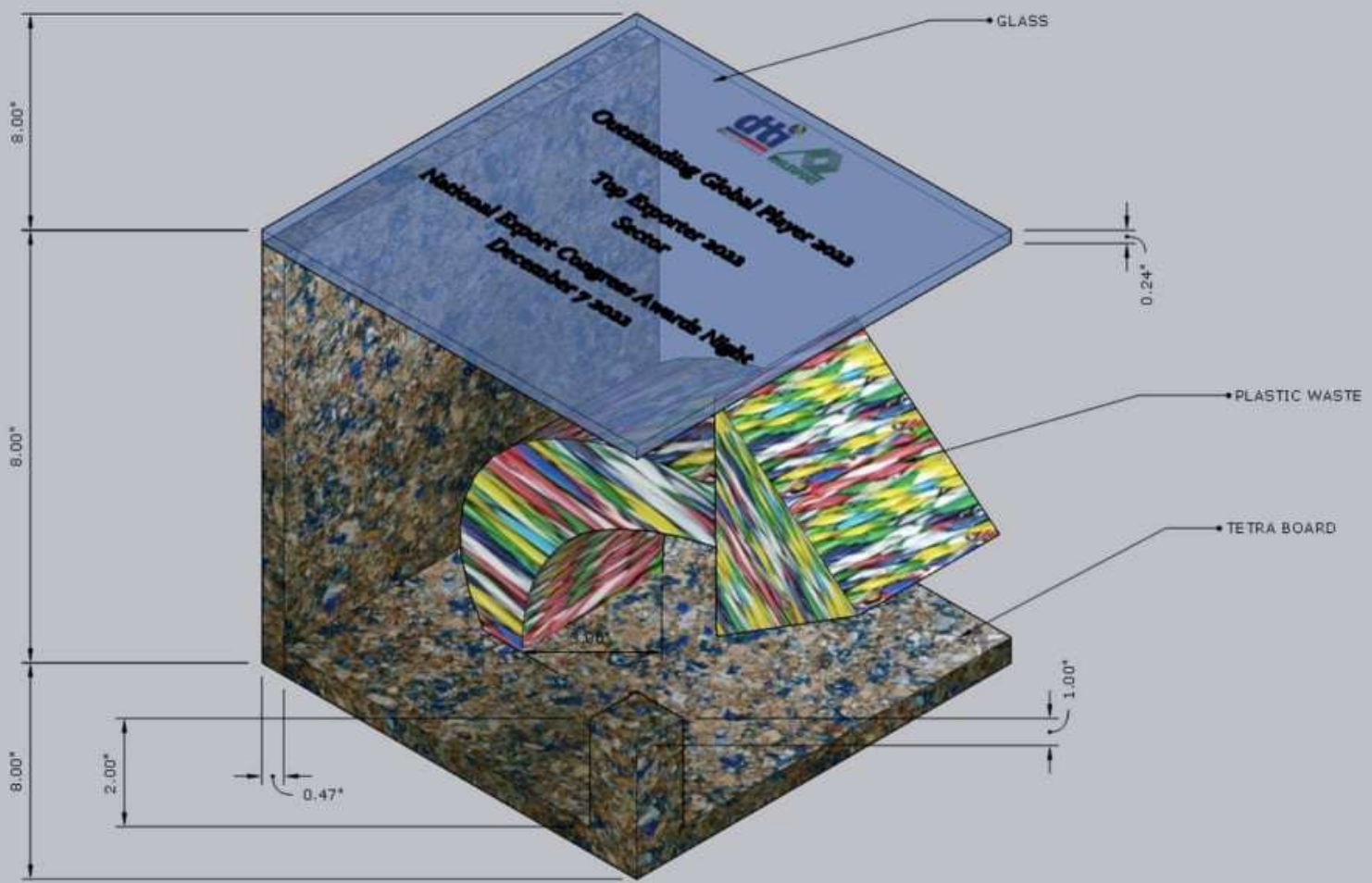
ISOMETRIC VIEW
